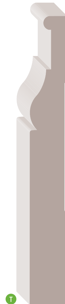
BAS-5C9 11/16" x 5-1/4" AP
