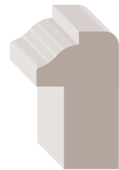
BAC-102 3/4" x 1-1/4" RABBET: 1/4" x 3/4"
